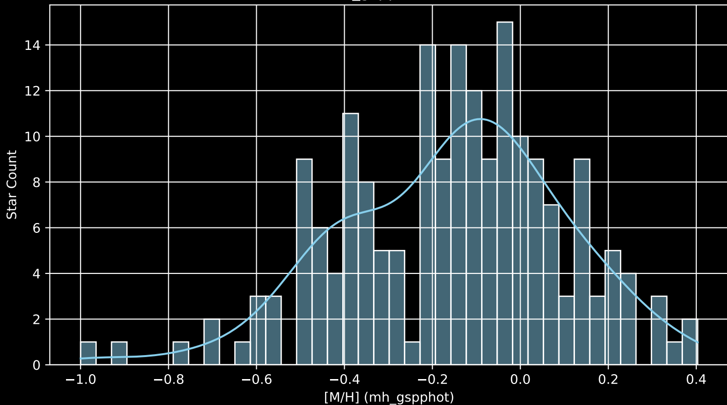
APOGEE DR17 Field: [267-34-O_TESS [M/H] (mh_gspphot) (n= 190)
