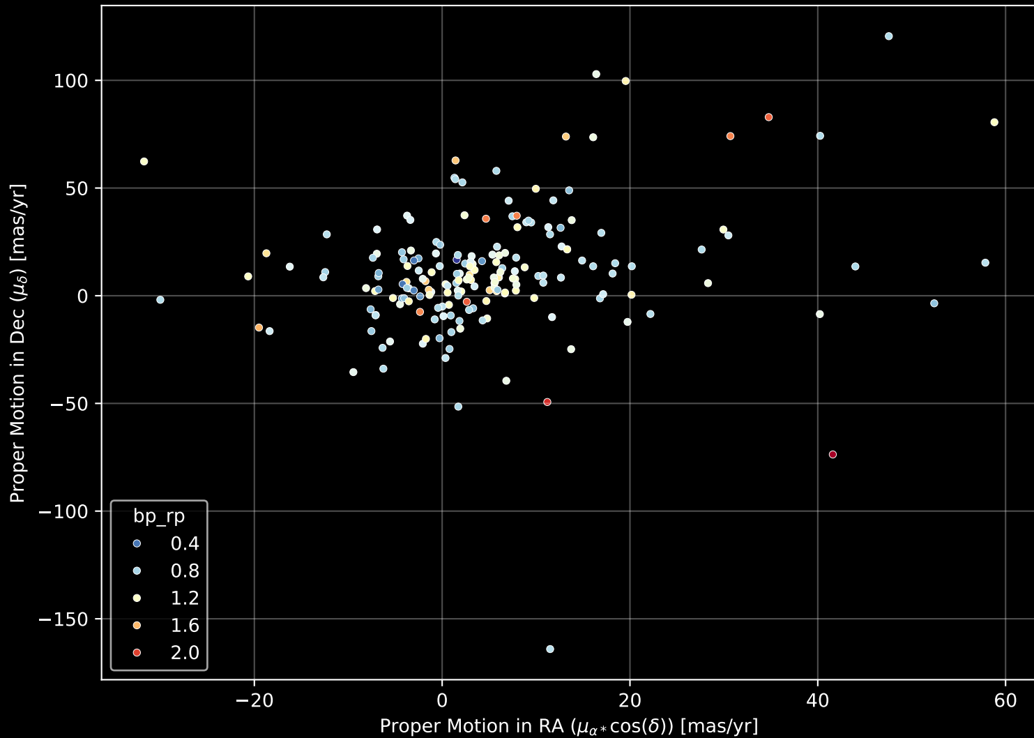
APOGEE DR17 Field: [267-34-O_TESS] Proper Motion Diagram (n= 192)
