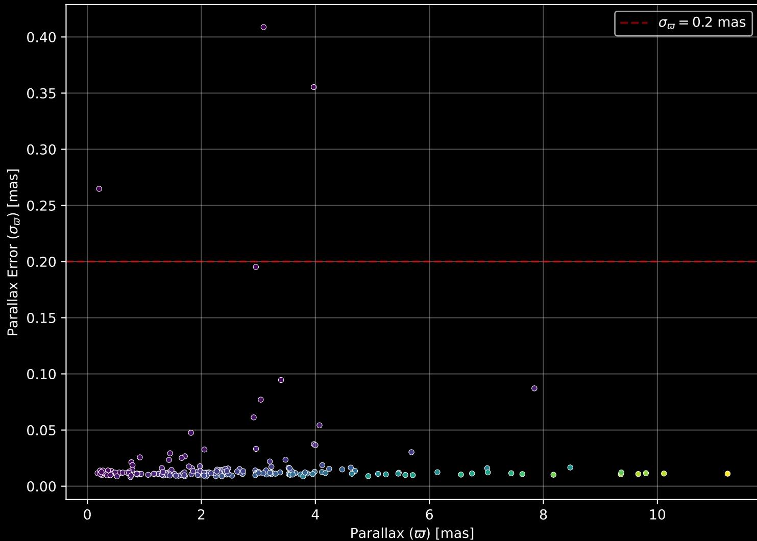
APOGEE DR17 Field: [267-34-O_TESS] Parallax Quality (n= 192)
