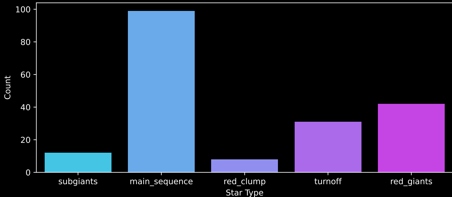
APOGEE DR17 Field: [267-34-O_TESS] Count plot of Star Type
