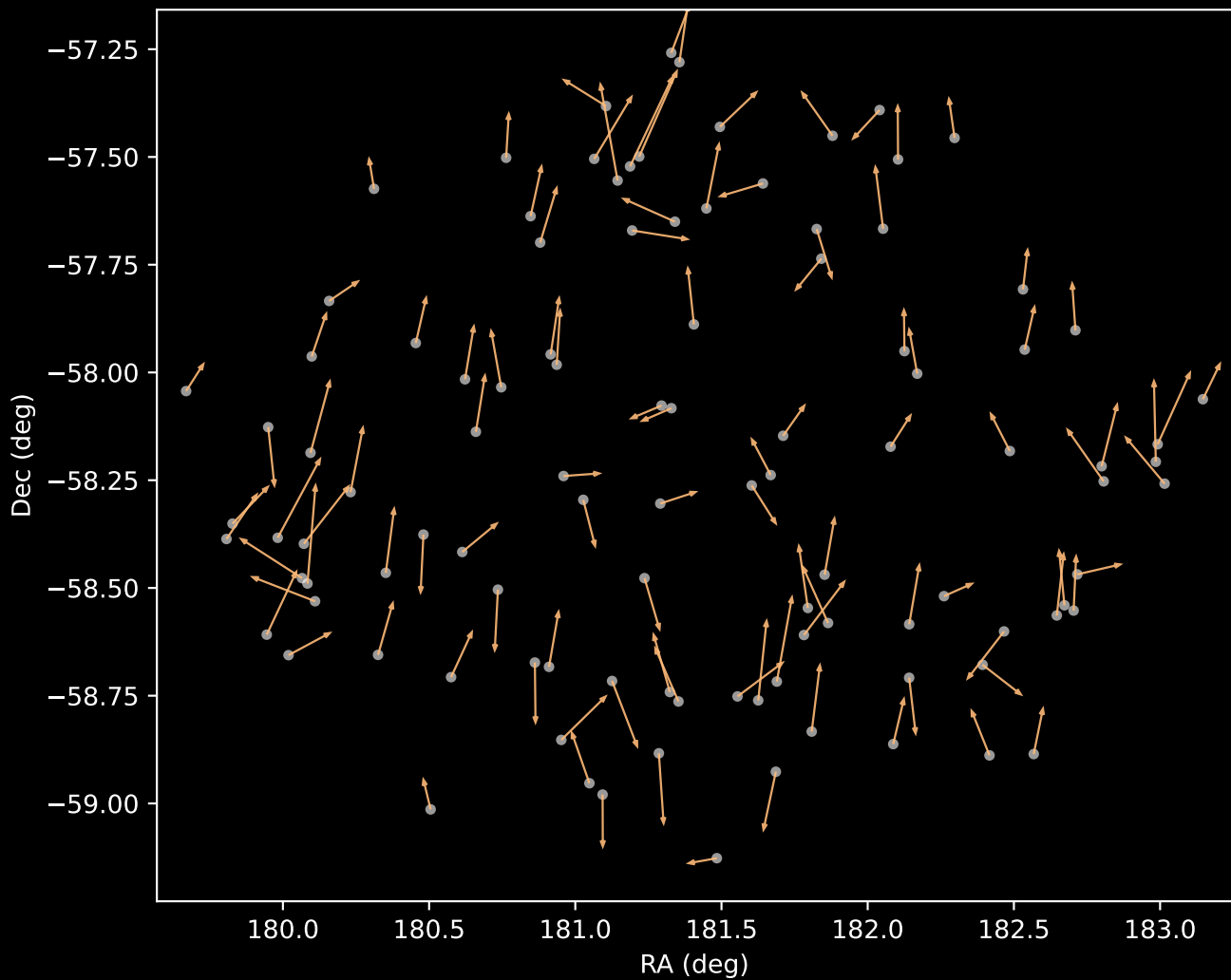
APOGEE DR17 Cluster 3 Proper Motion Vectors (n=105)
