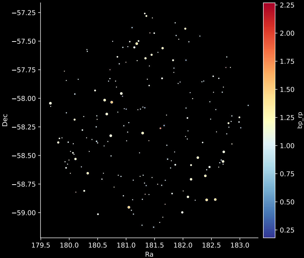
APOGEE DR17 Field: [267-34-O_TESS] Stars: 192
