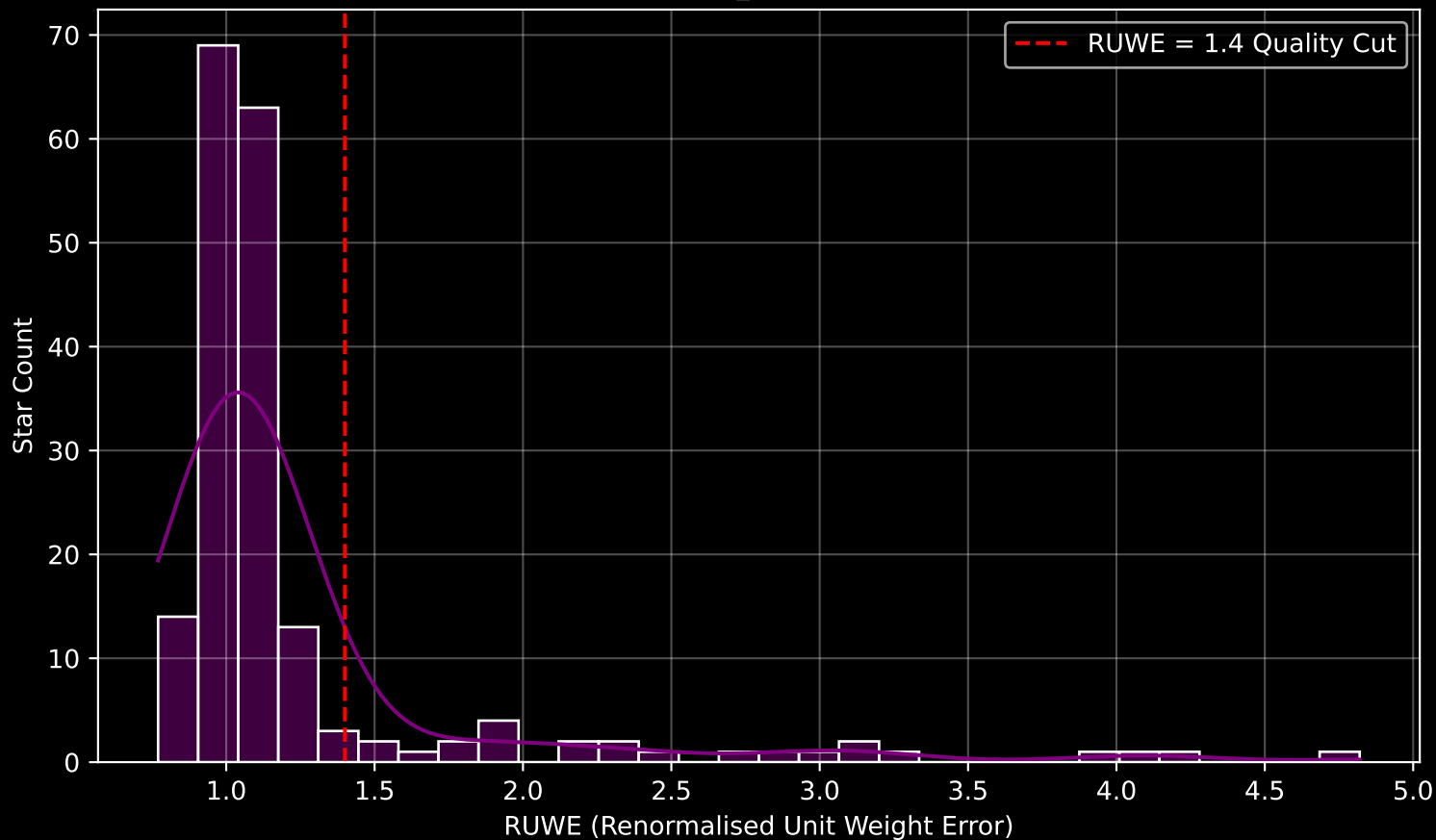
GAPOGEE DR17 Field [267-34-O_TESS] RUWE Distribution (n= 186)
